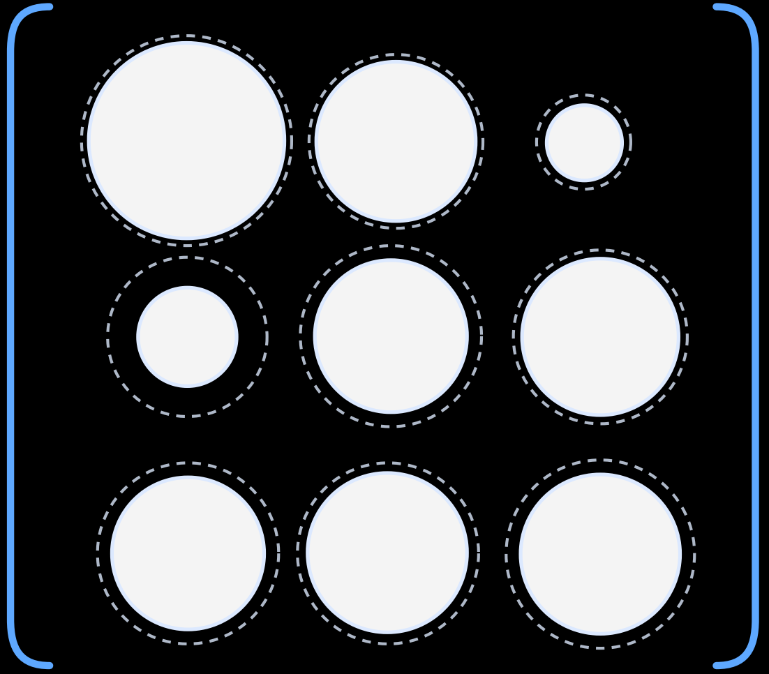
PMNS Matrix
